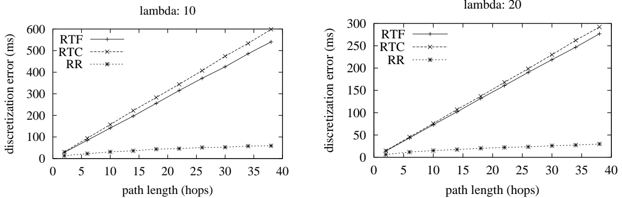
Fig. 1. Compare the average discretization errors of RTF, RTC and RR with respect to different path lengths. The vertical axis is the average of |\Delta^f(P)| , |\Delta^c(P)| , or |\Delta^r(P)| over 10000 sample paths.
