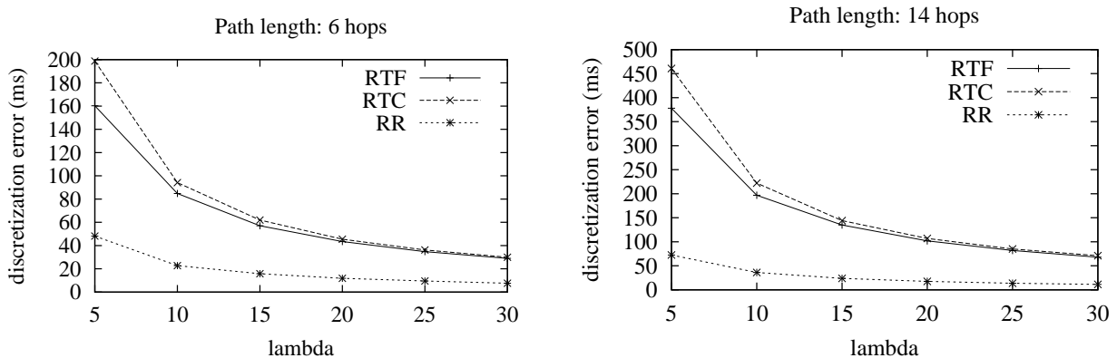
Fig. 2. Compare the average discretization errors of RTF, RTC and RR with respect to different \lambda values. The vertical axis is the average of |\Delta^f(P)| , |\Delta^c(P)| , or |\Delta^r(P)| over 10000 sample paths.
